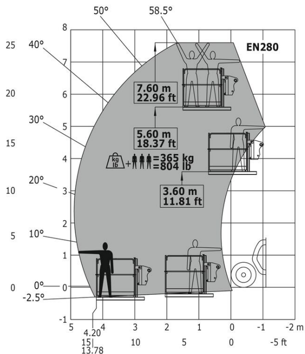
Machine on stabilizers with Man basket Metric
